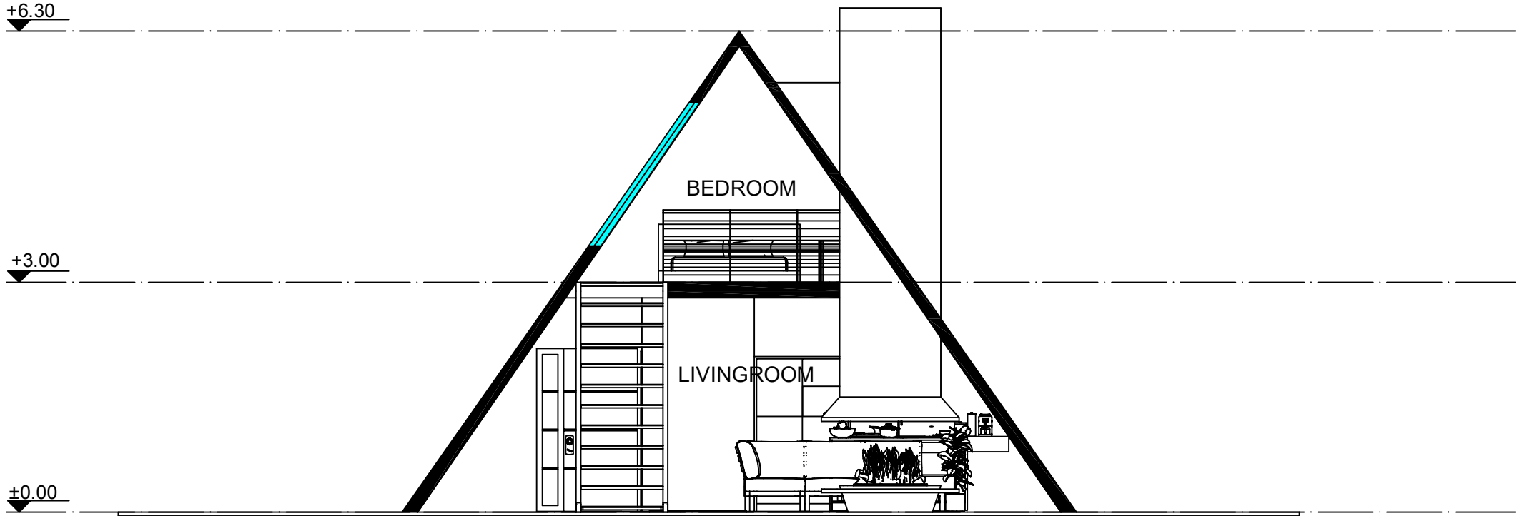
SECTION II-II
