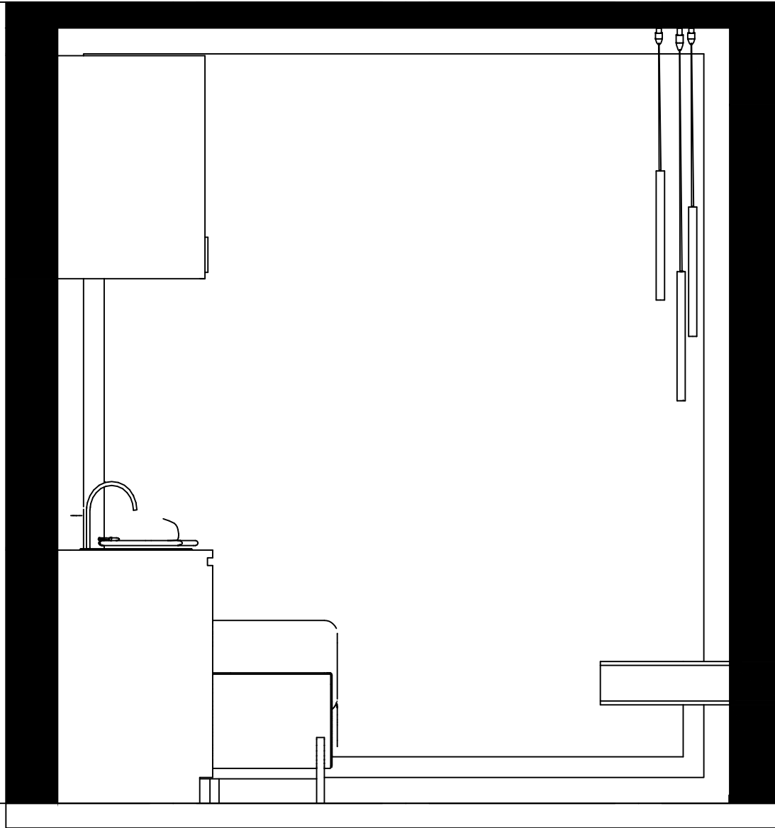
SECTION II-II
